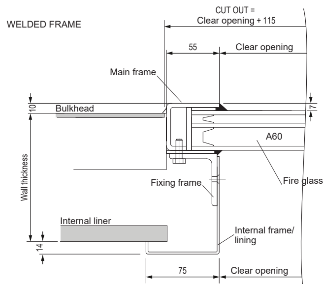
Welded frame designs:
